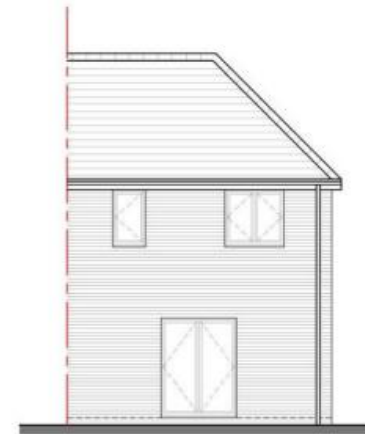
REAR ELEVATION
