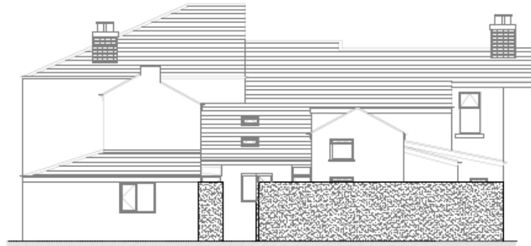
EXISTING REAR ELEVATION | SCALE 1:50
