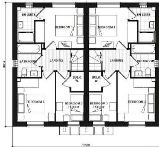
372 FIRST FLOOR PLAN
